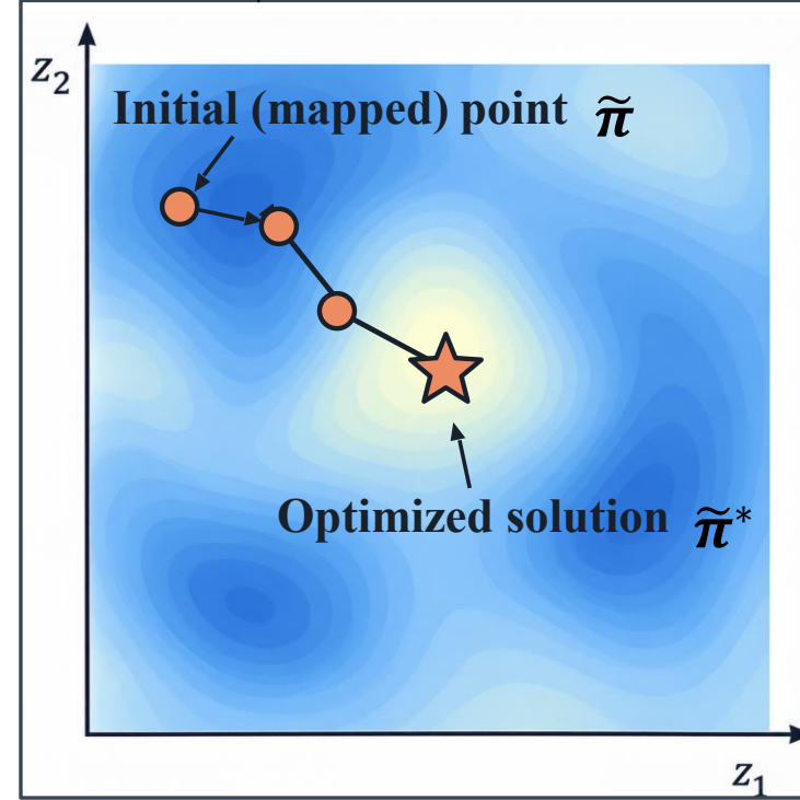
Compact solution space \Omega(\tilde{\mathbf{I}})
