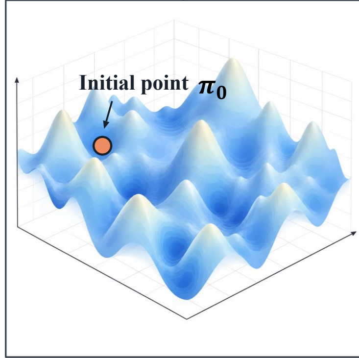
Original solution space \Omega(\mathbf{I})
